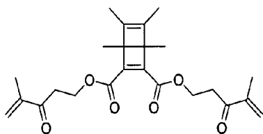
bis(4-methyl-3-oxopent-4-enyl) 1,4,5,6-tetramethylbicyclo[2.2.0]hexa-2,5-diene-2,3-dicarboxylate
