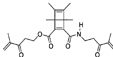
4-methyl-3-oxopent-4-enyl 1,4,5,6-tetramethyl-3-(4-methyl-3-oxopent-4-enylcarbamoyl)bicyclo[2.2.0]hexa-2,5-diene-2-carboxylate
