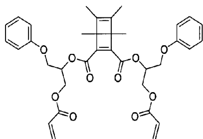
bis(1-(acryloyloxy)-3-phenoxypropan-2-yl) 1,4,5,6-tetramethylbicyclo[2.2.0]hexa-2,5-diene-2,3-dicarboxylate
