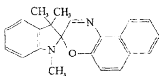
1,3-Dihydro-1,3,3-trimethylspiro[2H-indole-2,3'-[3H]naphth[2,1-b][1,4]oxazine]
