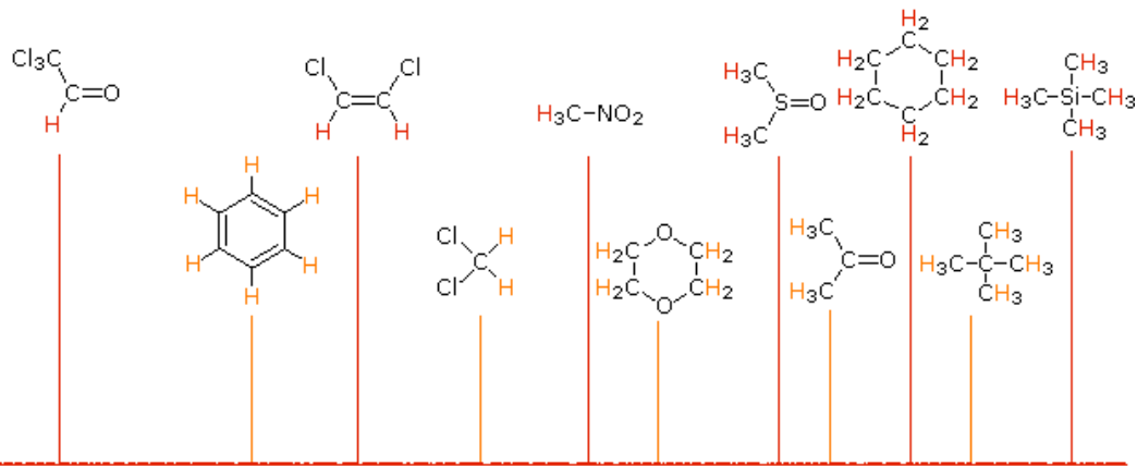
^1\text{H} NMR Resonance Signals for some Different Compounds
