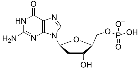
2'-deoxyguanosine 5'-phosphate
