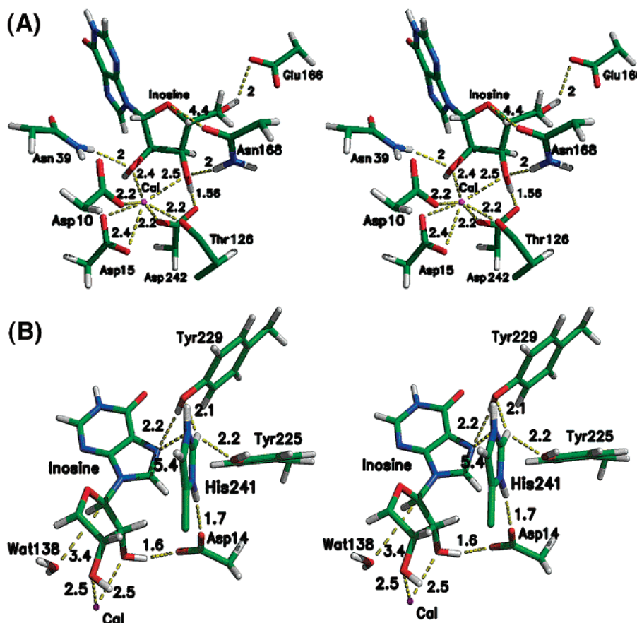
Figure 2. (A) Stereoimage of the active site residues of native EH·S interacting with the ribose part of inosine. Calcium is shown in magenta, hydrogen in white, carbon in green, oxygen in red, and nitrogen in blue. This represents the average structure from the MD simulation of EH·S. (B) Stereoimage of the active site residues of native EH·S showing the hydrogen bonding pattern between inosine, Asp14, Tyr225, Tyr229, and His241. Calcium is shown in magenta, hydrogen in white, carbon in green, oxygen in red, and nitrogen in blue. This represents the average structure from the MD simulation of EH·S.
