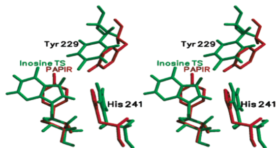
Figure 11. Stereomage comparing the position of His241-Tyr229-ligand from X-ray (2MAS) and average structure from EH•TS MD simulation. Note that Tyr229 in X-ray is closer to pAPIR as compared to His241.
