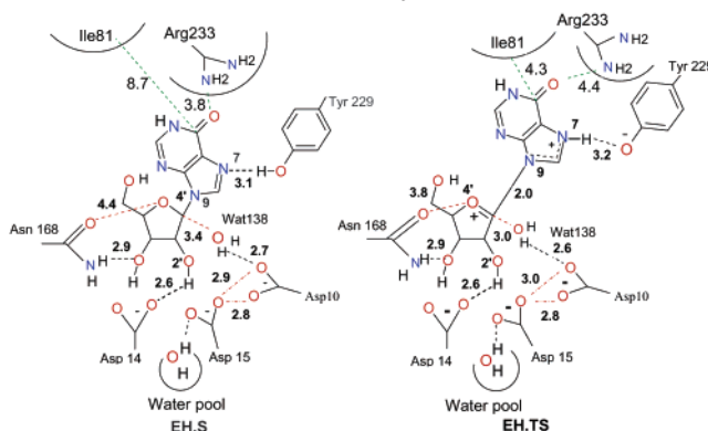
Chart 2. Putative Residues for Catalysis a
