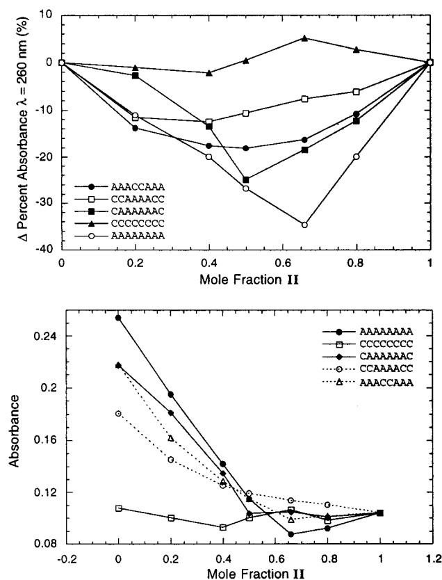
Figure 8. Job plots for DNG II with DNAs III , V , VI , IX , and XV plotted by percent hyperchromicity (top) and absorbance (bottom). [oligomer] = 2.0 μM, [KHPO 4 ] = 10 mM, [KCl] = 0.1 M, pH 7.4, observed at 260 nm.
