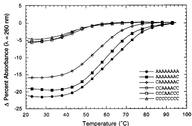
Figure 3. Thermal denaturation plots for DNA:DNG association (1.25 \mu M DNA oligomer, 2.5 \mu M DNG II , 10 mM KHPO 4 buffer, pH 7.4, 0.1 M KCl). Rate of heating was 0.2 ^{\circ} C/min DNA oligomer. Absorbance measurements taken every 1 ^{\circ} C (for clarity only one in five data points are represented by a symbol) in plots 1 through 4. DNA oligomer: III , ●; IV , ■; V , ◇; VI , ○; VII , □; and XV , △.
