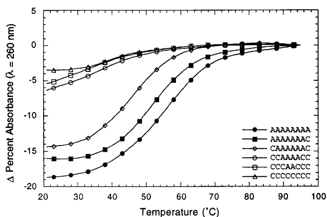
Figure 5. Thermal denaturation plots for DNA:DNG association (1.25 \mu M DNA oligomer, 2.5 \mu M DNG II , 10 mM KHPO 4 buffer, pH 7.4, 0.3 M KCl). Rate of heating was 0.2 ^{\circ} C/min DNA oligomer: III , ●; IV , ■; V , ◇; VI , ○; VII , □; and XV , △.
