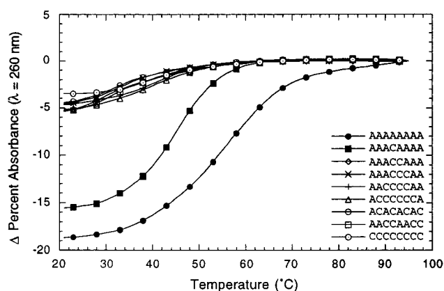
Figure 6. Thermal denaturation plots for DNA:DNG association (1.25 \mu M DNA oligomer, 2.5 \mu M DNG II , 10 mM KHPO 4 buffer, pH 7.4, 0.3 M KCl). Rate of heating was 0.2 ^{\circ} C/min DNA oligomer: III , ●; VIII , ■; IX , ◇; X , ○; XI , ×; XII , +; XIII , ○; XIV , □; and XV , ◆.
