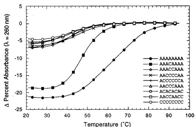
Figure 4. Thermal denaturation plots for DNA:DNG association (1.25 \mu M DNA oligomer, 2.5 \mu M DNG II , 10 mM KHPO 4 buffer, pH 7.4, 0.1 M KCl). Rate of heating was 0.2 ^{\circ} C/min DNA oligomer: III , ●; VIII , ■; IX , ◇; X , ○; XI , ×; XII , +; XIII , ○; XIV , □; and XV , ◆.
