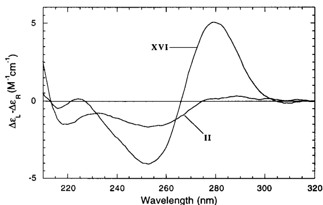
Figure 9. CD spectra of HO-T(pT) 7 -OH (○) compared to DNG II (●). Solution conditions: 2.0 × 10 -6 M oligomer, 0.1 M KCl, 10 mM phosphate buffer, pH 7.3 at 20 °C.
